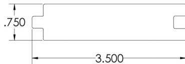
★ Net: 3/4 x 3-1/2
