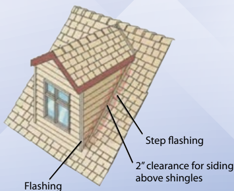
Figure 10 Typical dormer detail
