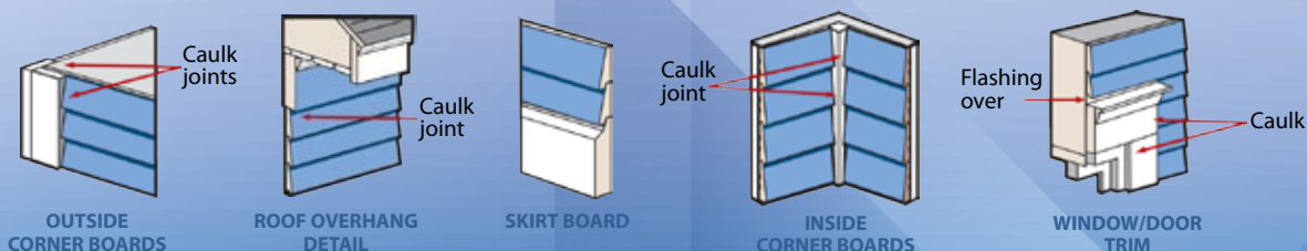
Figure 9 Typical trim details
