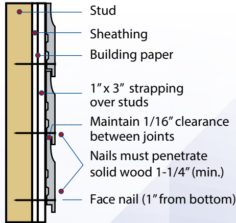
Figure 3 Cove Siding
