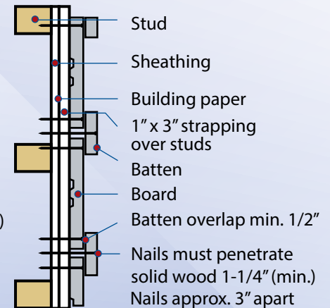
Figure 7 Board & Batten Siding (vert.)
